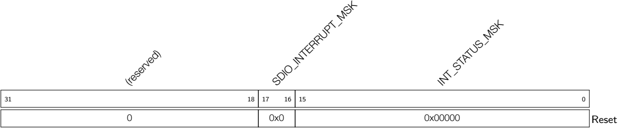
Register 9.19: MINTSTS_REG (0x0040)
