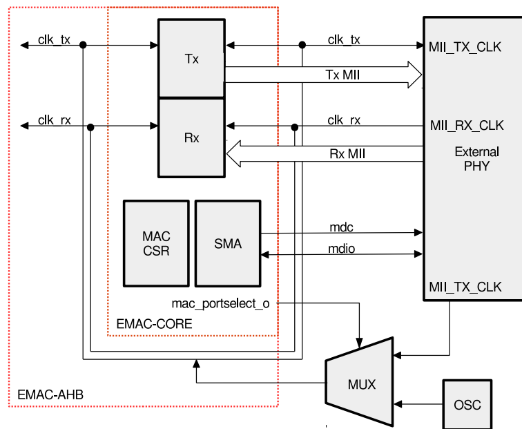
Figure 42: MII Clock
