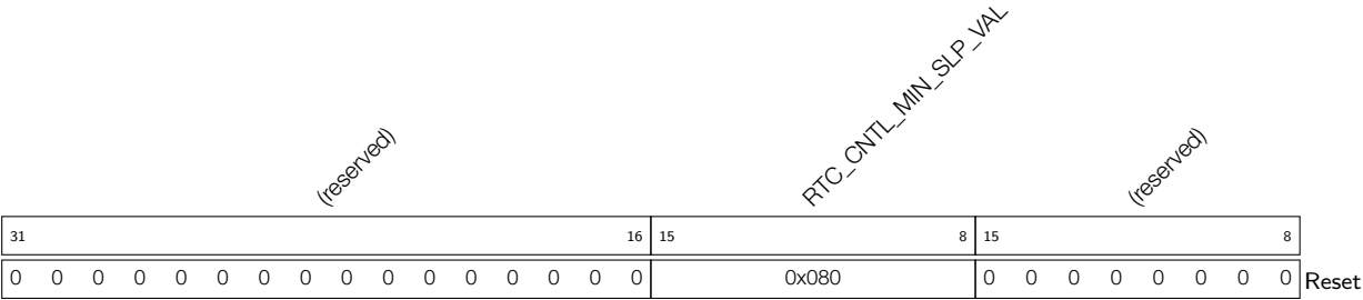
Register 30.10: RTC_CNTL_TIMER5_REG (0x000b)
