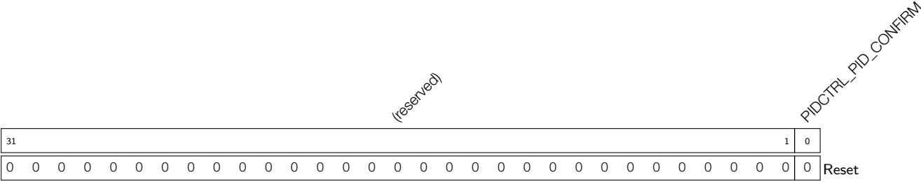
Register 27.14: PIDCTRL_PID_CONFIRM_REG (0x04C)
