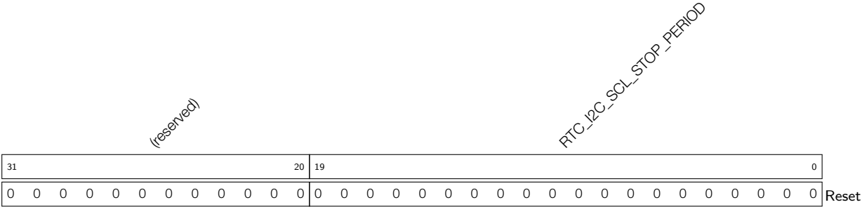
Register 29.19: RTC_I2C_SCL_STOP_PERIOD_REG (0x044)
