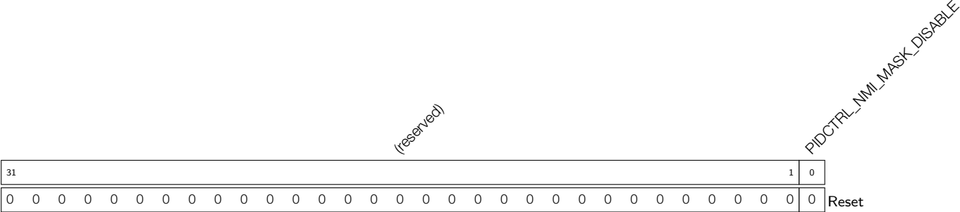
Register 27.16: PIDCTRL_NMI_MASK_DISABLE_REG (0x058)
