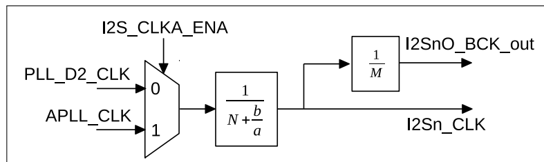
Figure 60: I2S Clock
