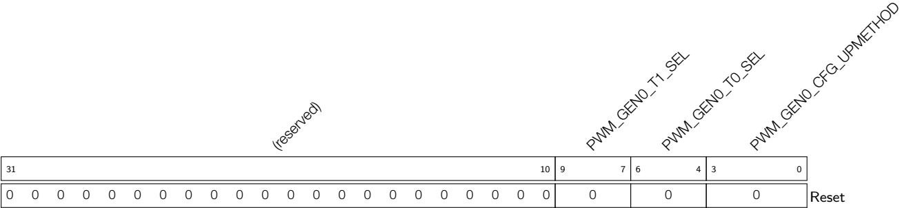
Register 16.19: PWM_GEN0_CFG0_REG (0x0048)
