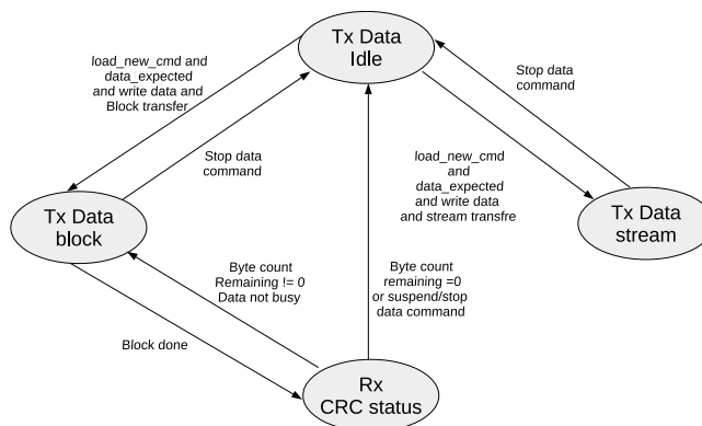
Figure 34: Data Transmit State Machine
