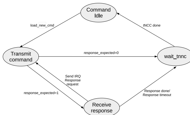
Figure 33: Command Path State Machine
