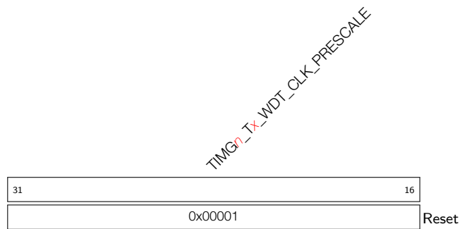
Register 18.11: TIMG n T x WDTCONFIG1_REG (0x004c)
