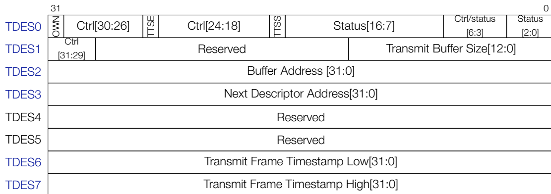
Figure 45: Transmit Descriptor
