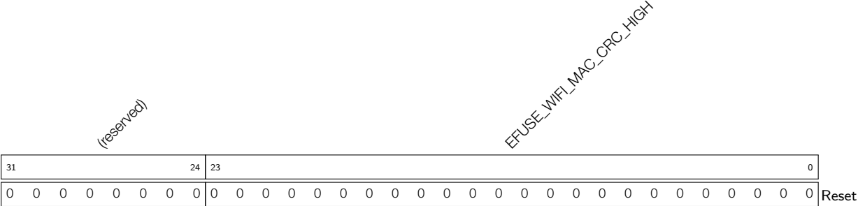
Register 20.10: EFUSE_BLK0_WDATA2_REG (0x024)
