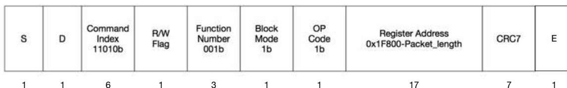
Figure 22: CMD53 Content
