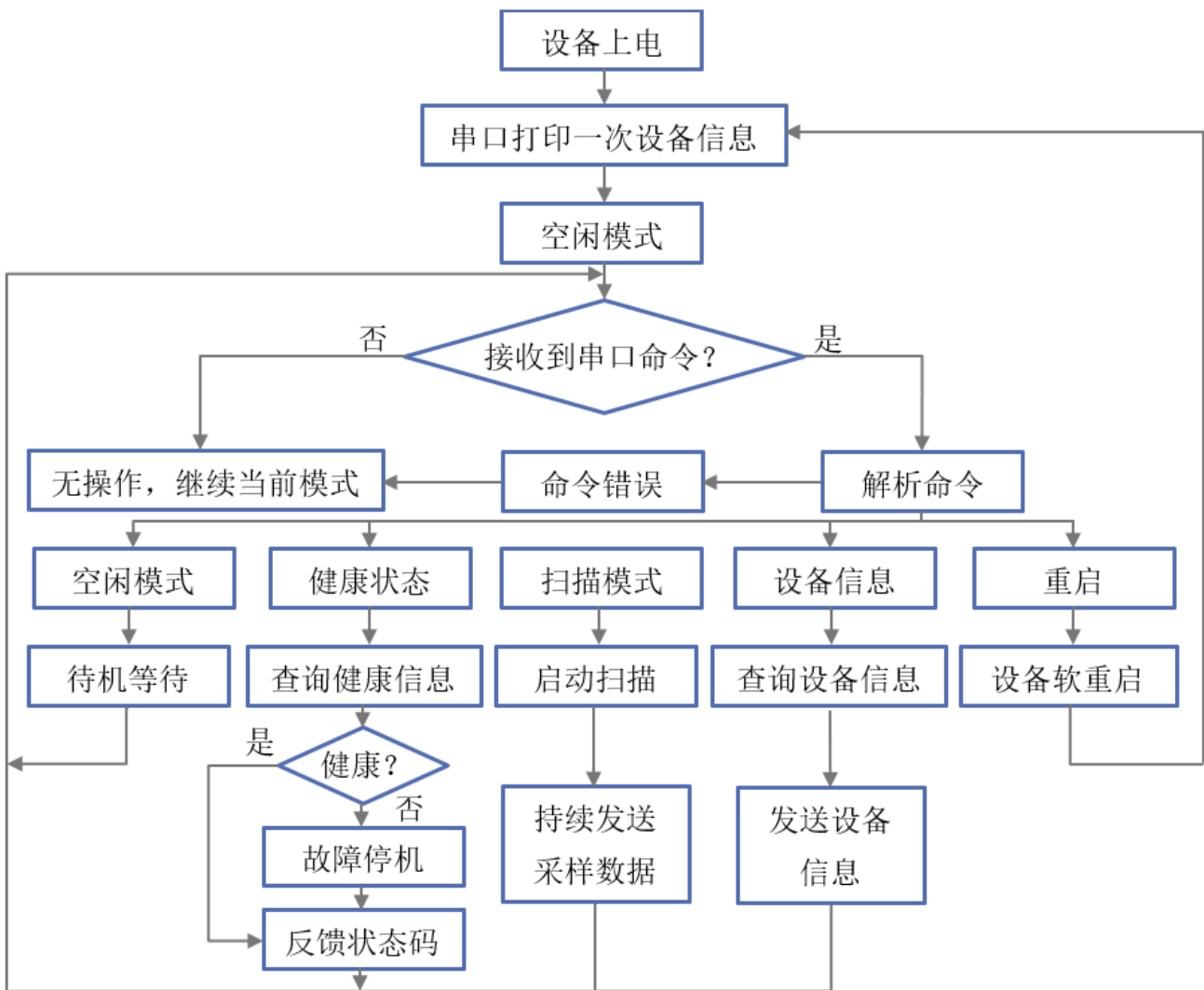
FIG 1 YDLIDAR X4 SYSTEM WORKFLOW
