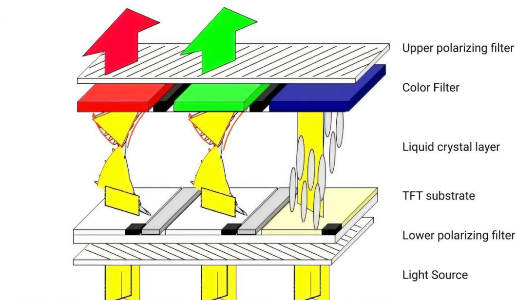
Display Screen CXM090IPS-D27 Schematic Diagram
