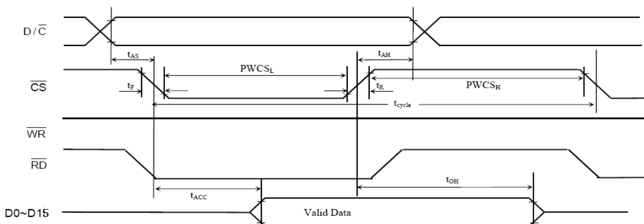
Figure 7. 80-system Bus Timing
