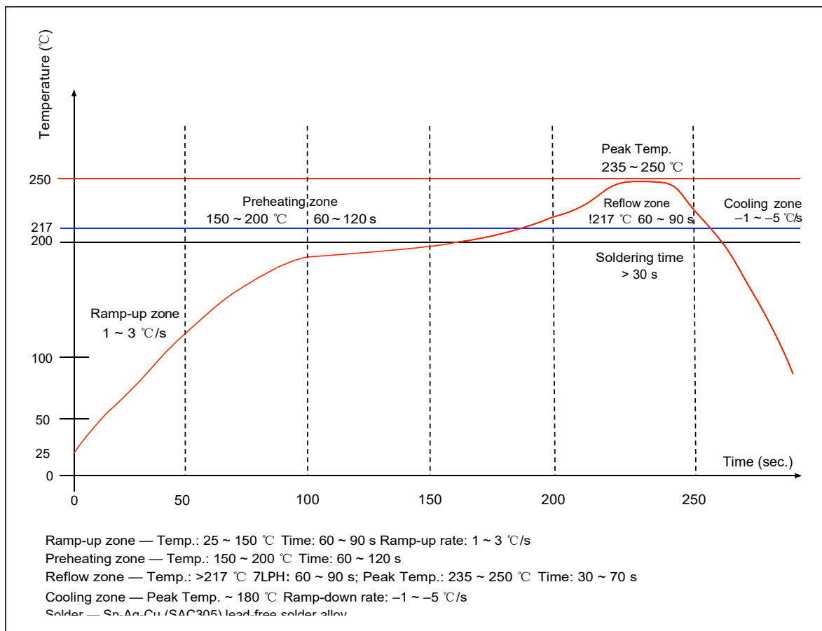
Figure 10: Reflow Profile
