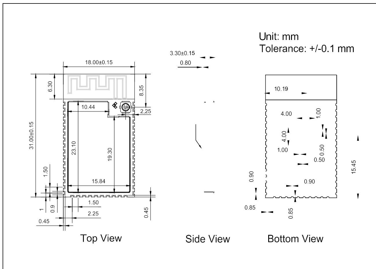
Figure 7: Physical Dimensions
