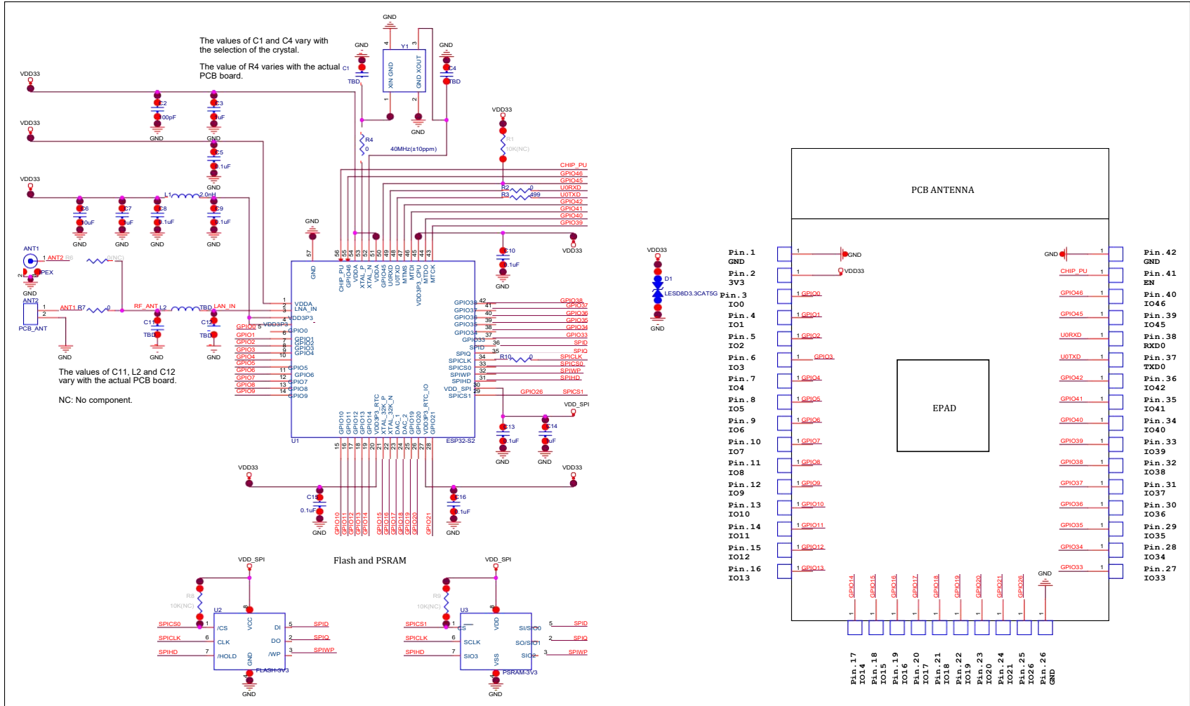
Figure 4: ESP32-S2-WROVER Schematics
