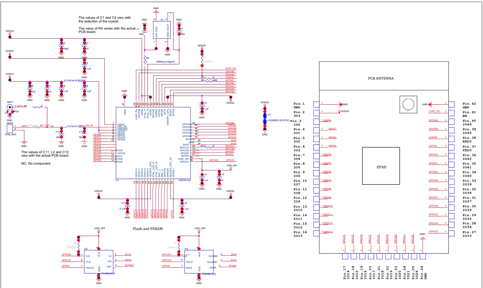
Figure 5: ESP32-S2-WROVER-I Schematics
