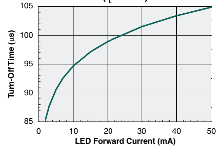
Typical Turn-Off vs. LED Forward Current ( I_L=75mA )
